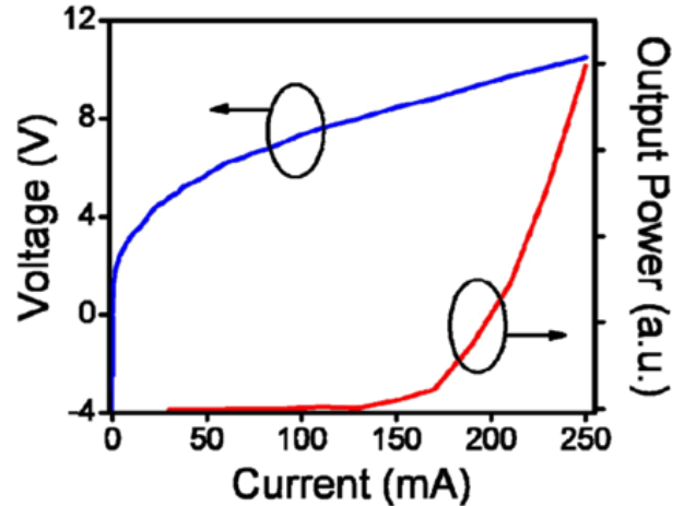
Figure 7: L-I and I-V curves of NSSP LED.
